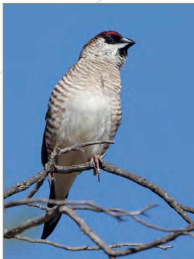
Neochmia (formes sauvages); Neochmia modesta – Diamant modeste
